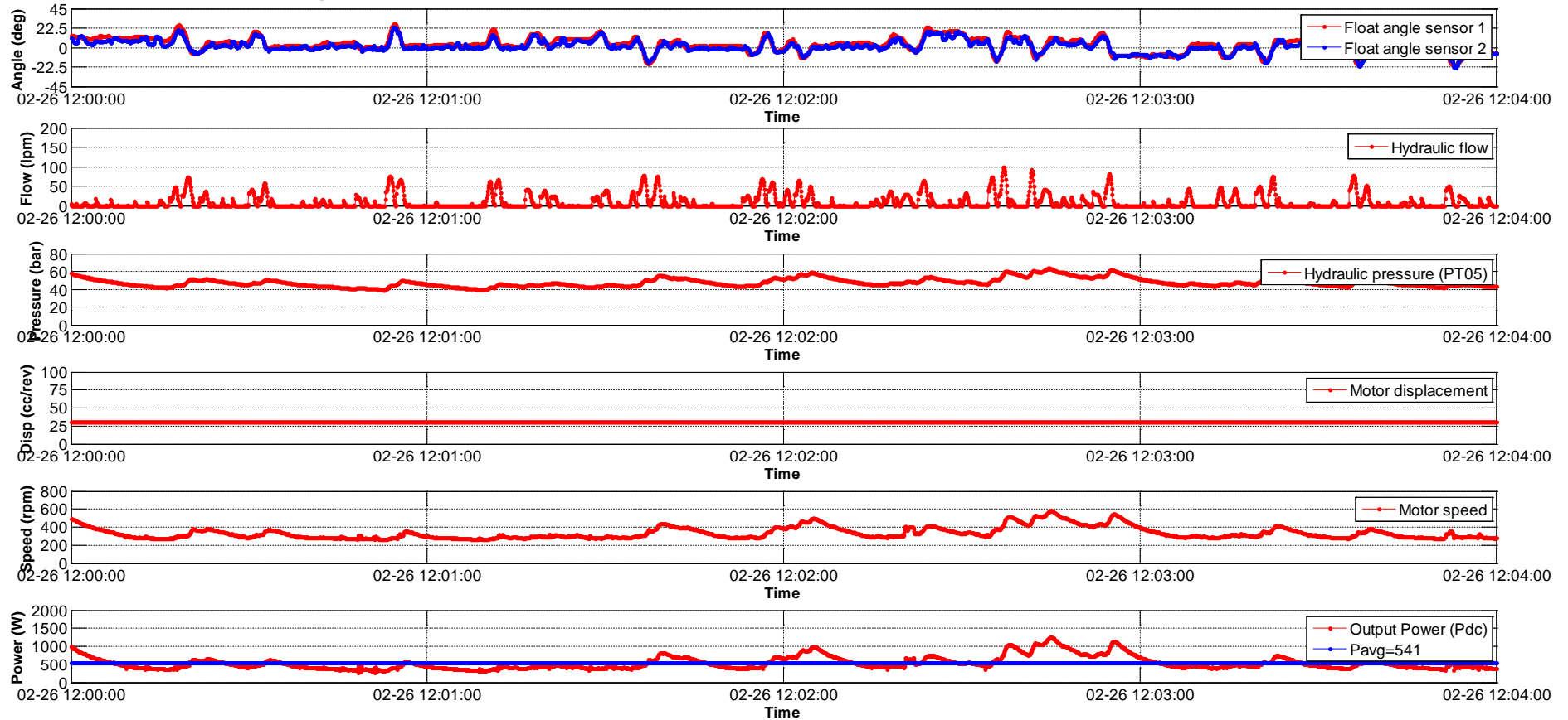
Float angle, flow, pressure, motor displacement, speed & power plots from file NWEI OfS 10Hz data 20160226 1200
