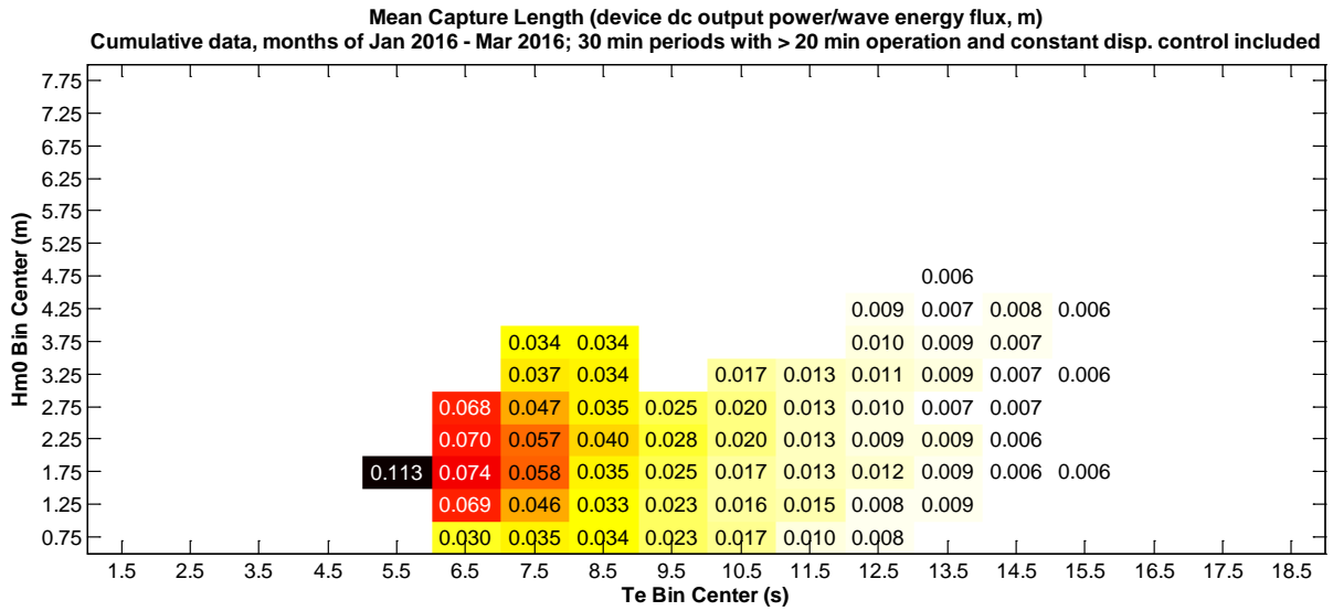
Figure 5-5 Mean capture length
