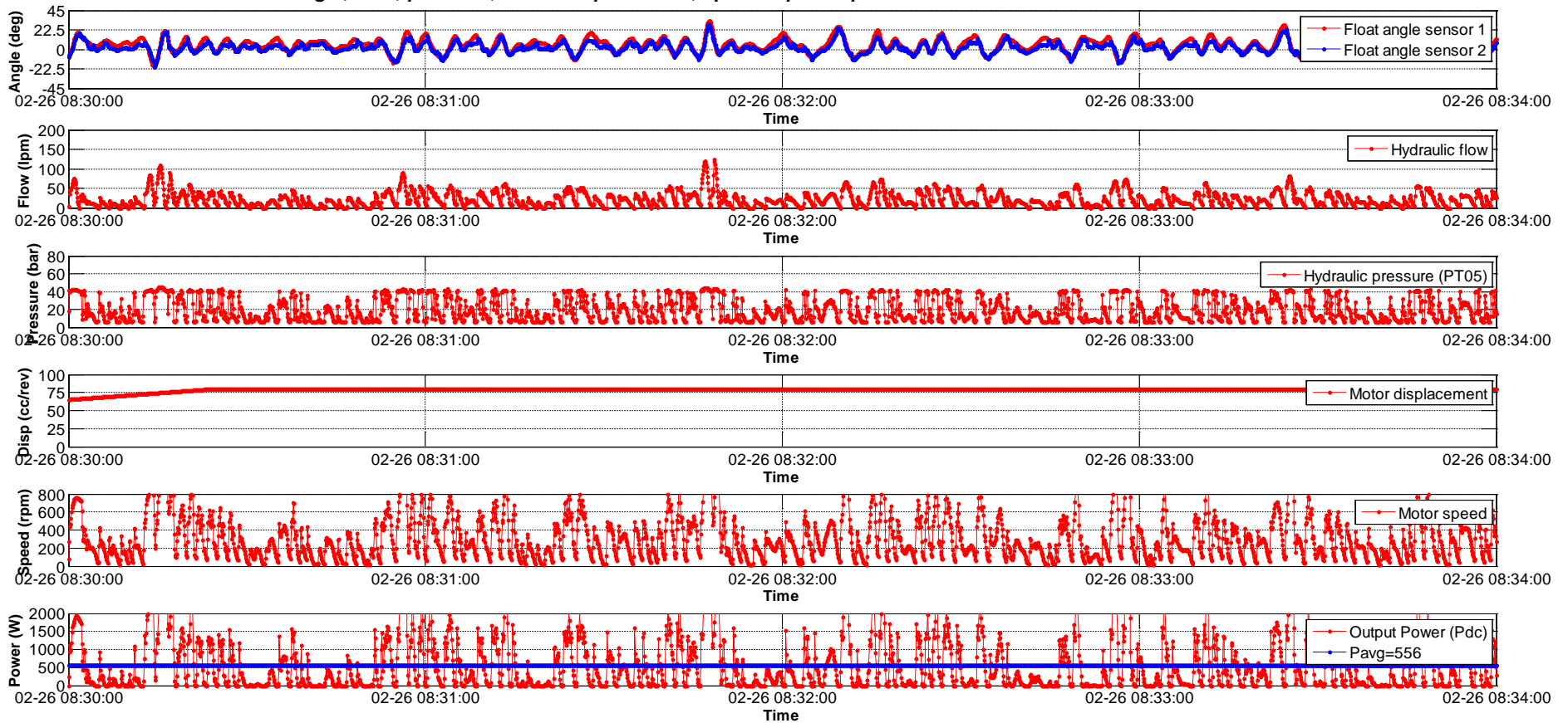
Float angle, flow, pressure, motor displacement, speed & power plots from file NWEI OfS 10Hz data 20160226 0830
